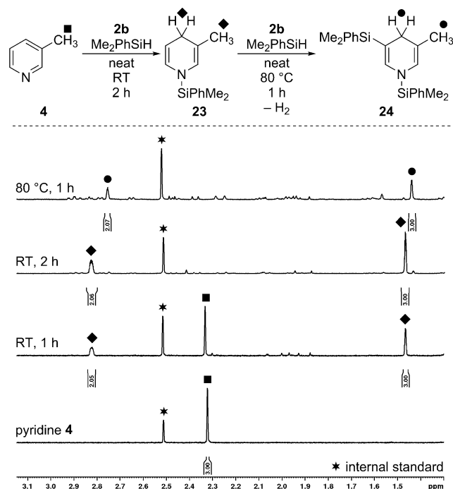
Scheme 4. Monitoring the C–H silylation of 3-picoline ( 4 ) by 1 H NMR spectroscopy (400 MHz) in CD 2 Cl 2 : detection of key intermediates.
