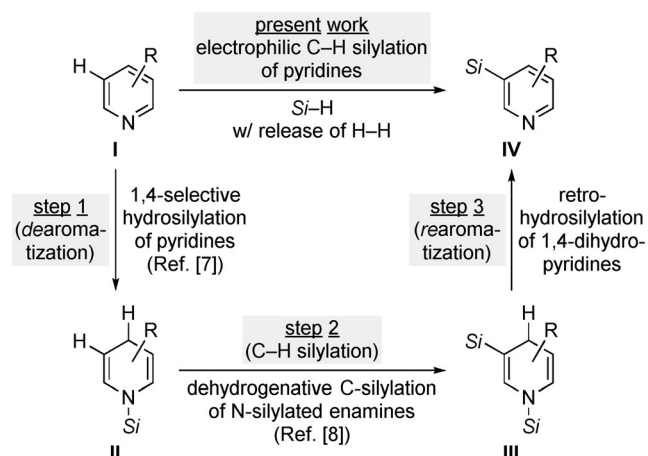
Scheme 1. Strategy for an electrophilic C–H silylation of pyridines that does not follow an S_EAr reaction at the pyridine nucleus. Si = triorgano-silyl.
