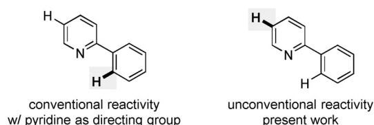
Figure 1. C–H bonds in 2-phenylpyridine ( 1 ) addressed by conventional (left) and unconventional (right) C–H silylation.
