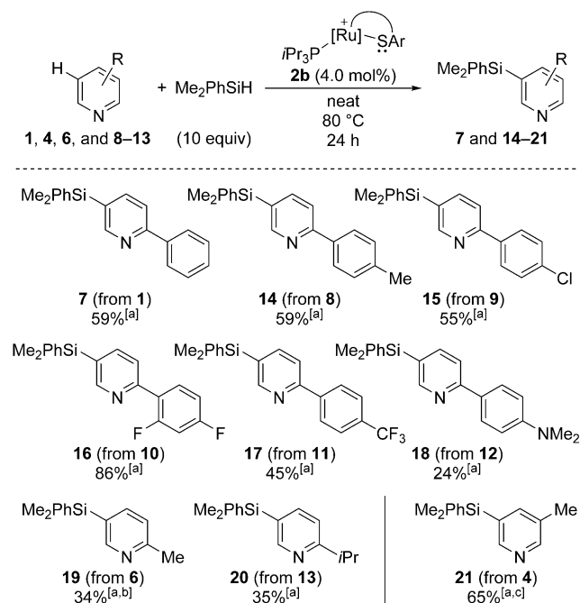
Scheme 3. 5-Selective C–H silylation of 2- and 3-substituted pyridines.
