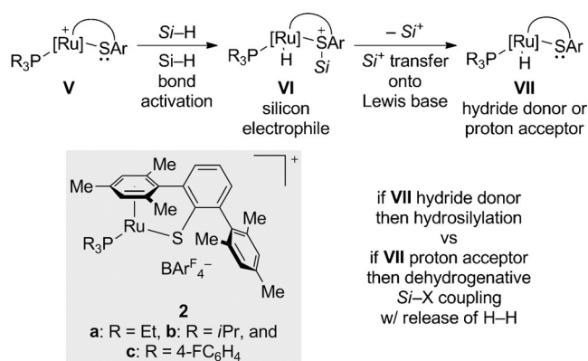
Scheme 2. Cooperative Si-H bond activation and silicon cation transfer (counteranion \text{BARF}_4^- omitted for clarity, top), and the tethered Ru-S complexes 2 tested as catalysts (bottom). \text{Ar}^F = 3,5\text{-bis(trifluoromethyl)phenyl} .
