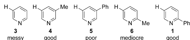
Figure 2. Performance of model compounds tested in the initial screening.
